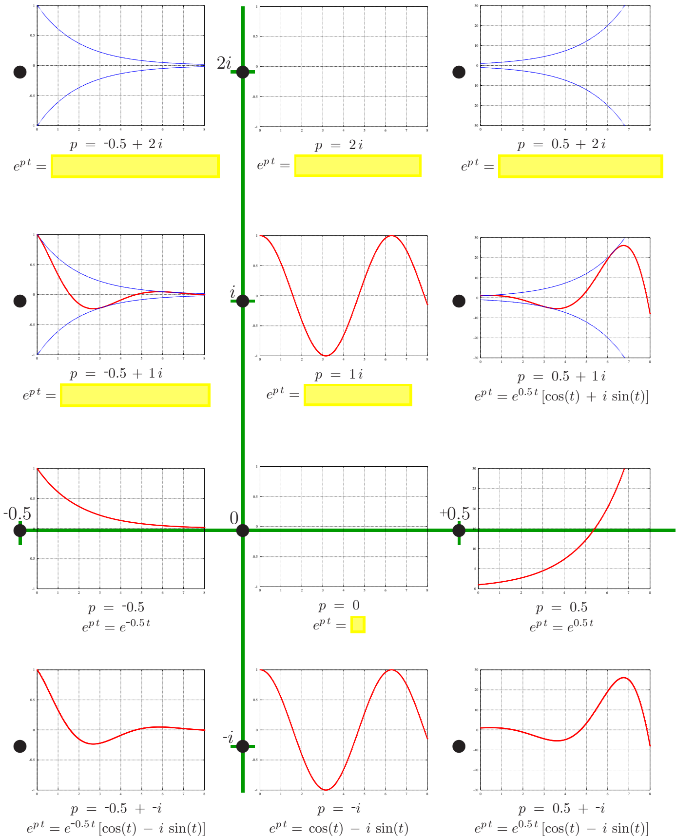
Figure 5.1: Pole location in the complex plane and behavior of e^{pt}
